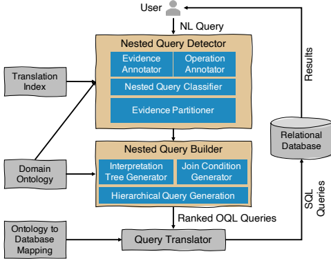
Figure 2: System Architecture
